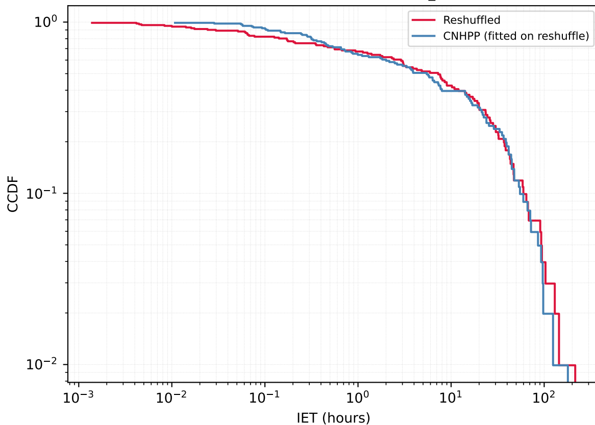
User 5357949 - Reshuffled vs CNHPP A_{\text{fit}}=0.6712
